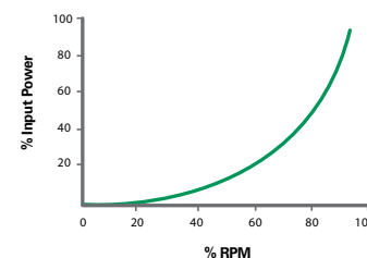
Pump Motor Speed vs. Power Consumption
